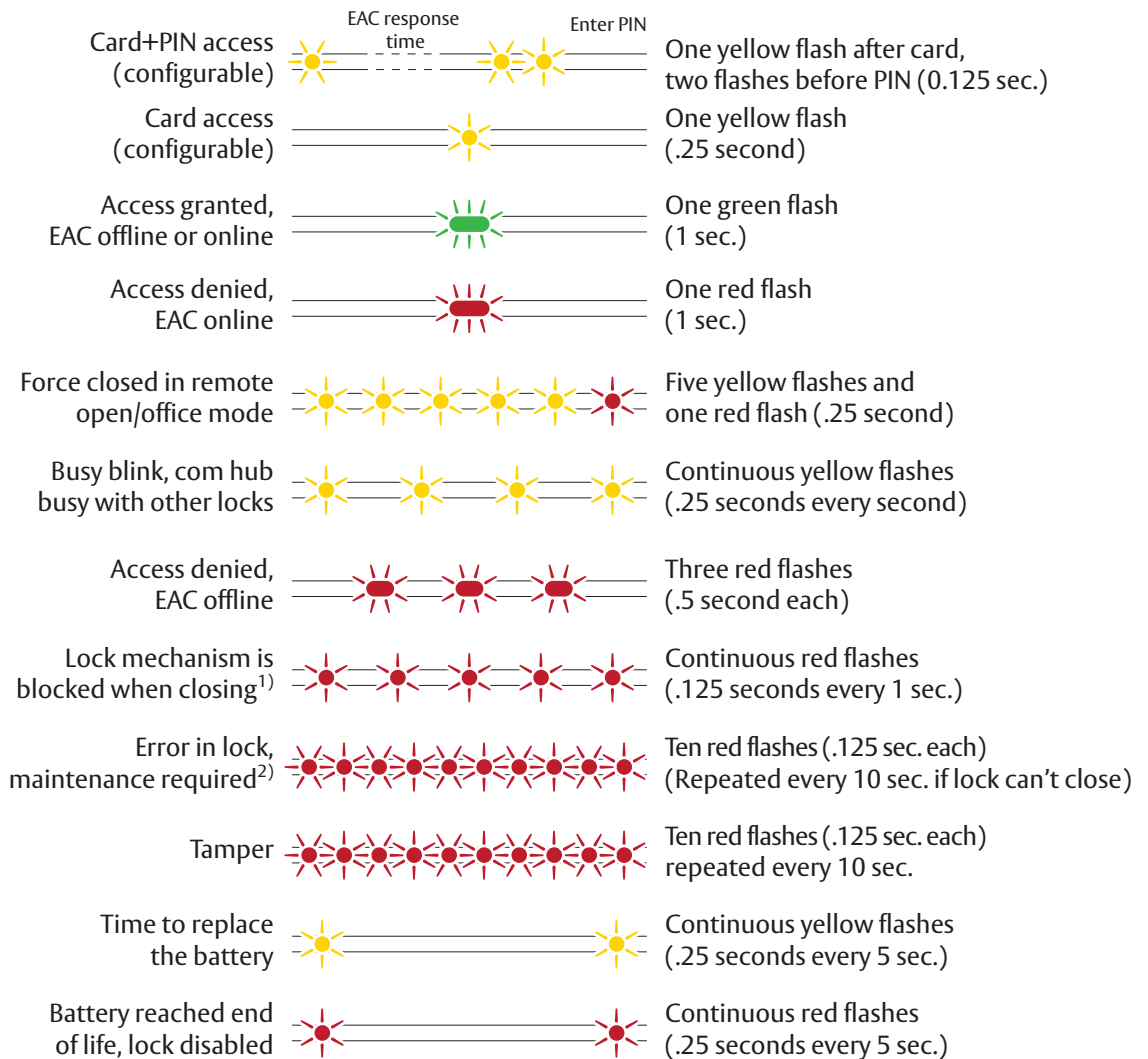
Figure 25. Lock normal operation LED indication
