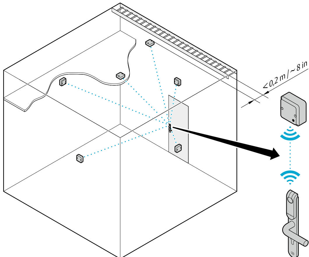
Figure 6. Placement options for AH20/30/40 communi- cation hub
