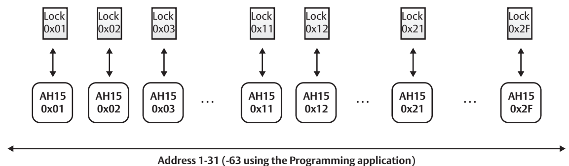
Figure 7. Address allocation in a default installation
