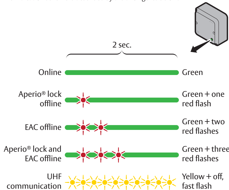
Figure 22. Communication hub normal operation LED indication
